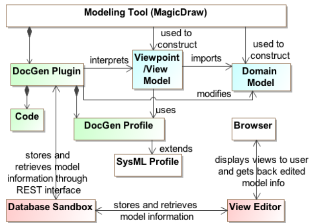
Figure 18. View Editor Components
